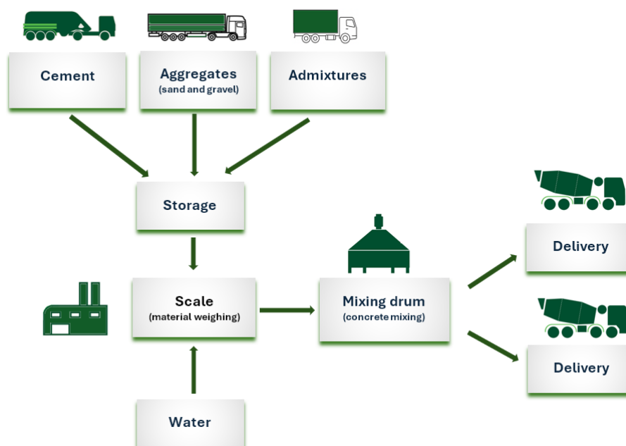
Figure 3 – The ready-mixed concrete manufacturing process
